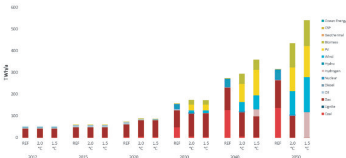
Figure 18: Breakdown of electricity generation by technology
