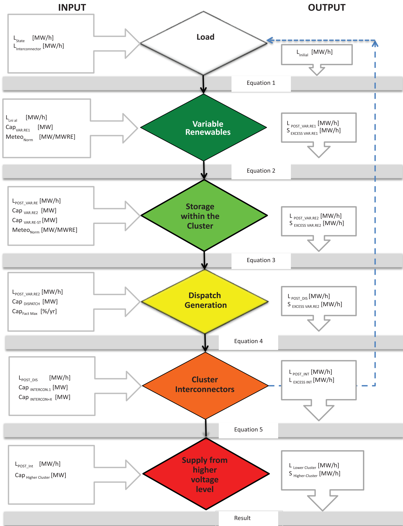
Figure 7: Overview: input, output and dispatch order
