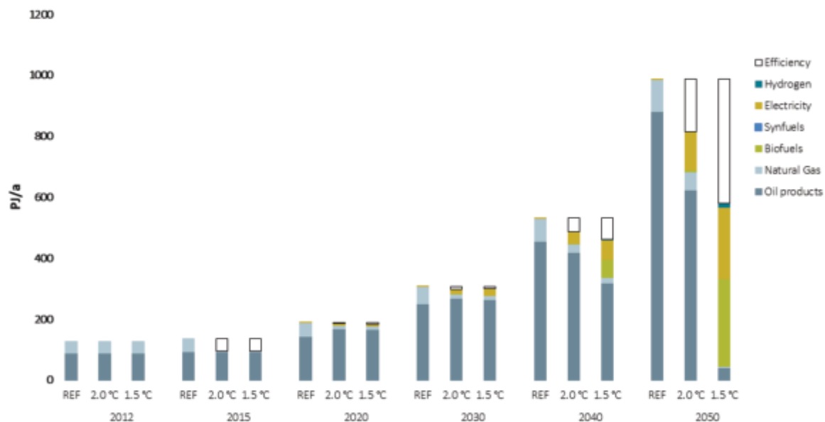
Figure 22: Final energy consumption transport under the scenarios
