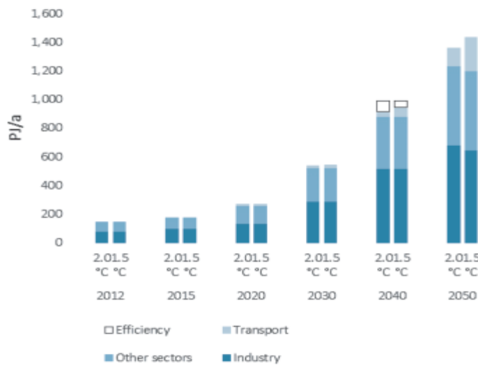
Figure 16: Development of electricity demand by sector in both RENEWABLES scenarios
