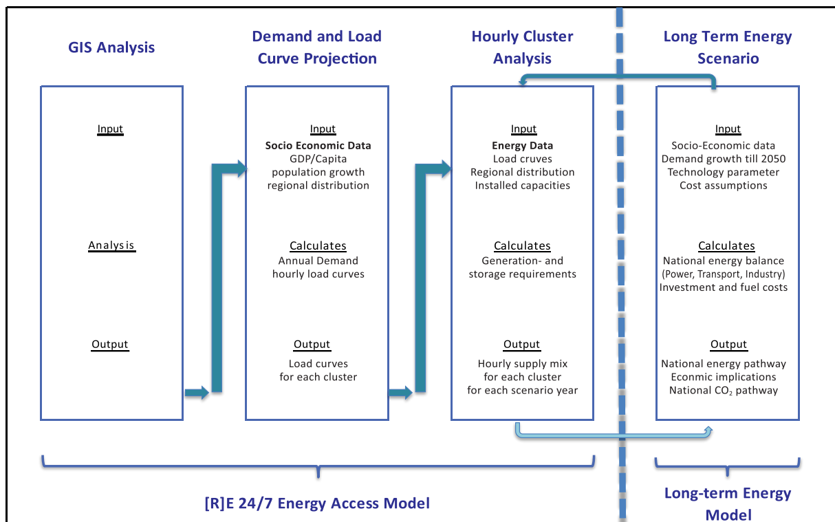
Figure 4: Overview – Modelling concept
