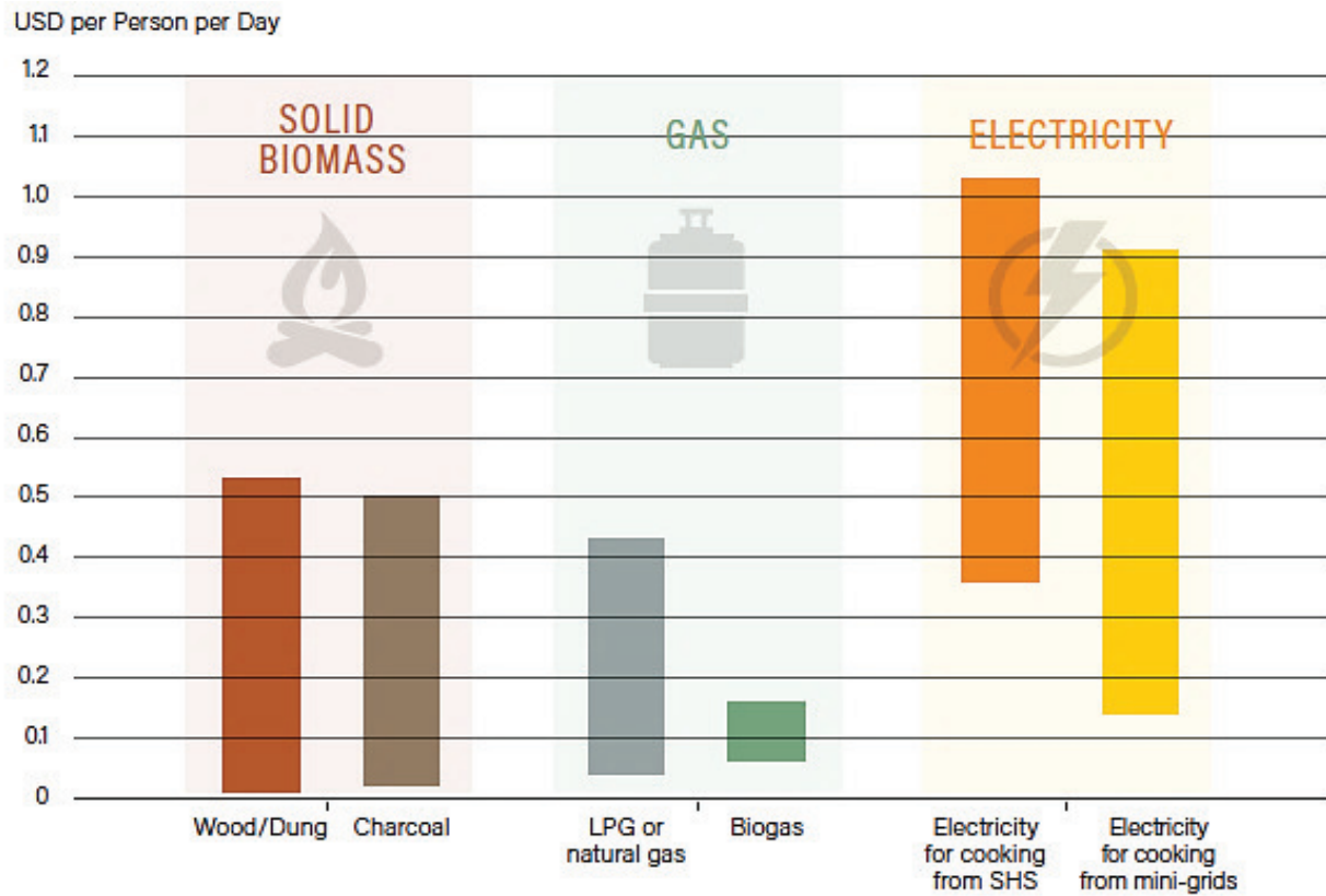
Figure 3: Costs of various cooking technologies (REN21 GSR 2017)
